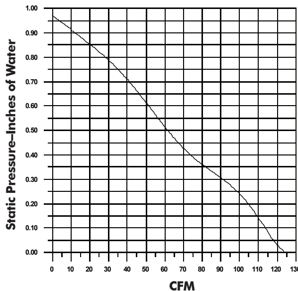
NuVent Product Performance Model NXSS120FL
